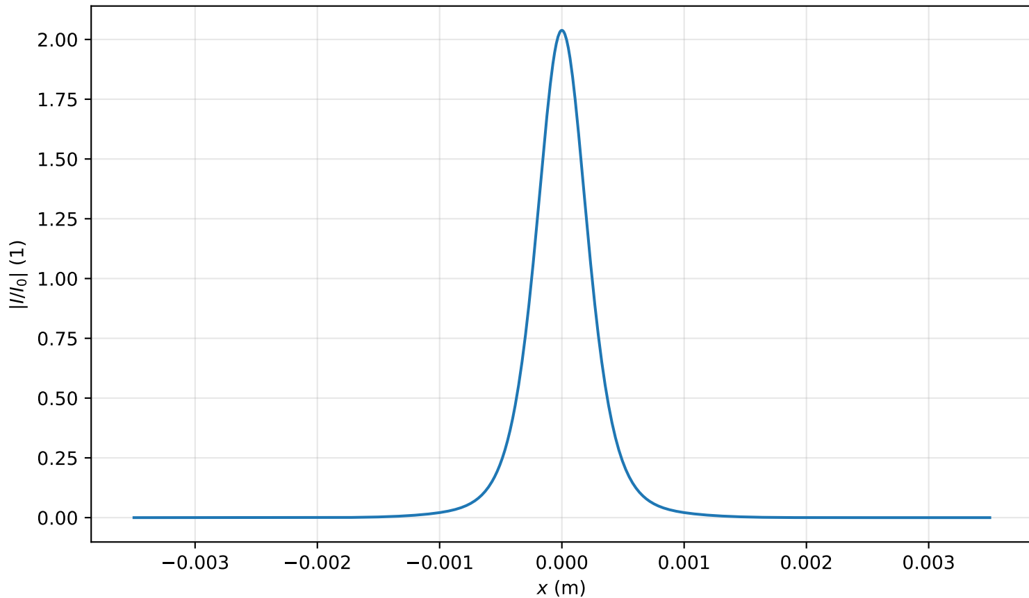
Intensity profile I(x, y = 0, z = 1.831m)/I_0 , P_{in}=1.0P_{cr} , artificial time
